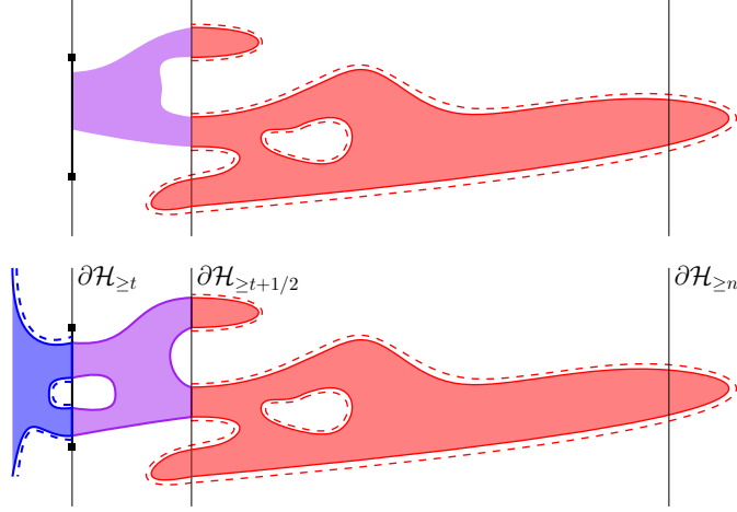
Figure 7: Top: A realisation \chi of C_{\geq 1/2} under \mathcal{L}_{n-t} in red, and the link in purple. Bottom: The same realisation, shifted by (Lt, X_t) as C_{\geq t+1/2} . The measure here is \phi[\cdot | C_{\leq t}, X_n \neq \dagger] . Note that the link is different in the two diagrams.
