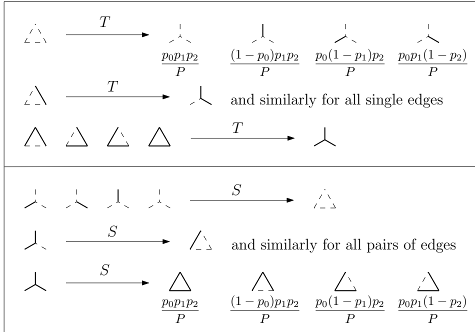
FIG 2.2. The ‘kernels’ T and S and their transition probabilities. The constant P is given by P := (1 - p_0)(1 - p_1)(1 - p_2) .
