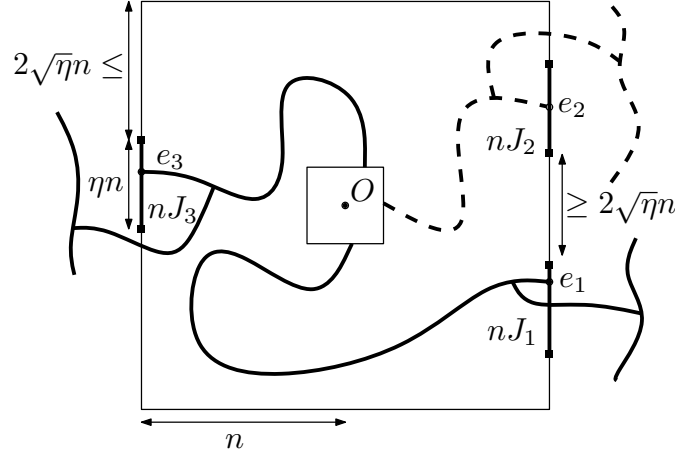
FIG 3.3. The event A_{\sigma}^{\varnothing, J}(N, n) with \sigma = (1, 0, 1) and \eta -landing-sequence J . Each crossing \Gamma_i is an \eta -exterior-fence with exterior endpoint e_i \in nJ_i .
