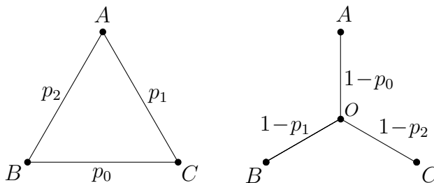
FIG 2.1. The star–triangle transformation when \kappa_{\Delta}(\mathbf{p}) = 0 .
