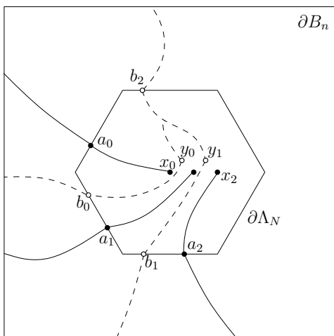
FIG 3.1. The vertices x_r (respectively, y_r ) may be connected by open (respectively, open*) paths to the a_r (respectively, b_r ) in such a way that the event A_6(n) results.
