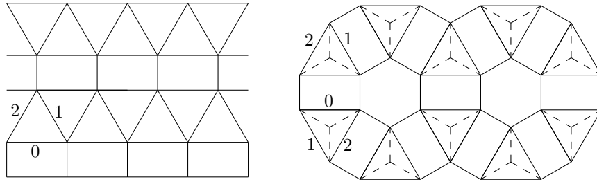
FIG 1.2. Isoradial embeddings of the Archimedean lattices (3^3, 4^2) and (3, 4, 6, 4) . The second may be transformed into the hexagonal lattice by one sequence of star-triangle transformations as marked. An edge parallel to one labelled i has edge-parameter p_i , and the two parameters on any square have sum 1.
