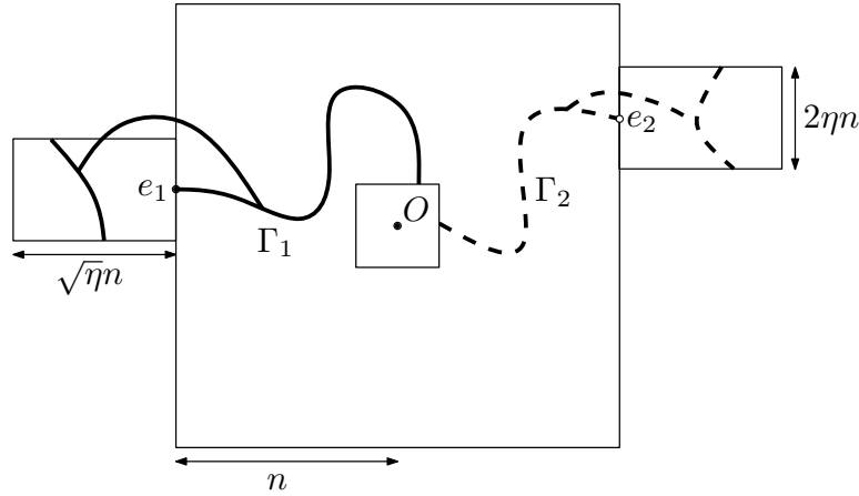
FIG 3.2. A primal \eta -exterior-fence \Gamma_1 with exterior endpoint e_1 , and a dual \eta -exterior-fence \Gamma_2 .
