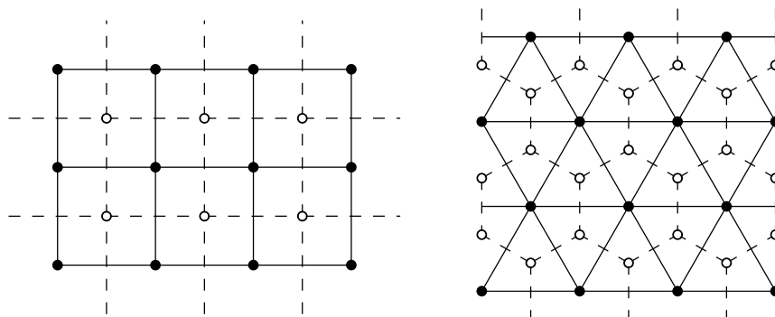
FIG 1.1. The square lattice and its dual square lattice. The triangular lattice and its dual hexagonal lattice.
