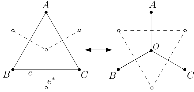
FIG 2.3. The star-triangle transformation acts simultaneously on primal and dual graph elements.
