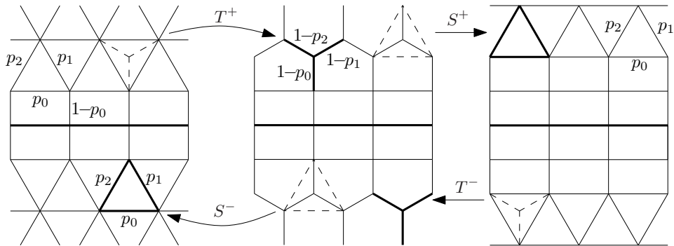
FIG 2.4. The transformation S^+ \circ T^+ (respectively, S^- \circ T^- ) transforms \mathbb{L}^1 into \mathbb{L}^2 (respectively, \mathbb{L}^2 into \mathbb{L}^1 ). They map the dashed graphs to the bold graphs.
