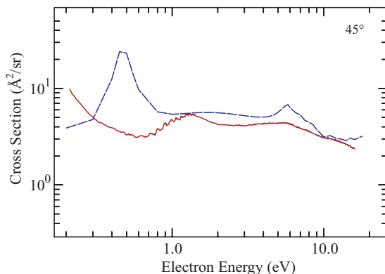
FIG. 2. (Color online) Elastic cross sections at 45^\circ .
