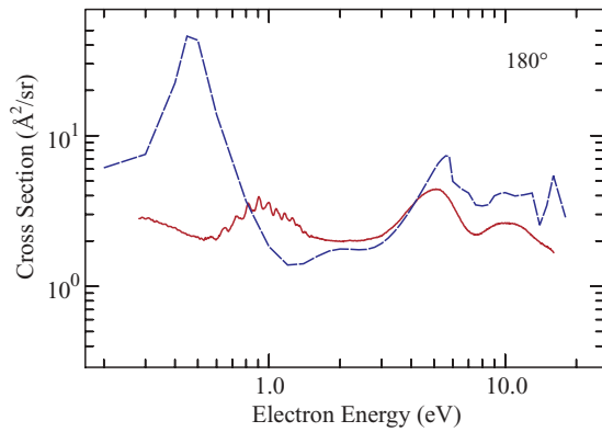
FIG. 5. (Color online) Elastic cross sections at 180^\circ .
