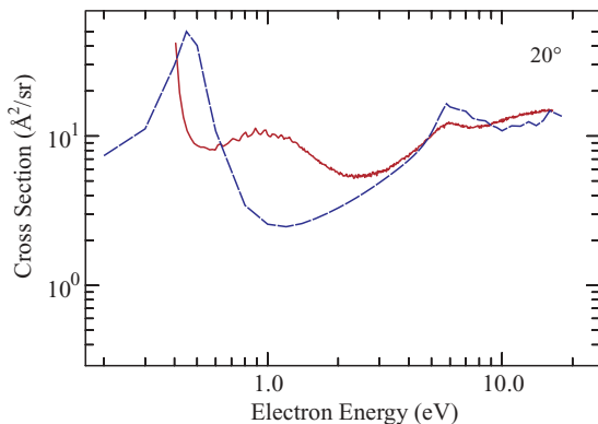
FIG. 1. (Color online) Elastic cross sections at 20^\circ . Solid (red) line, experiment; dashed (blue) line, theory.
