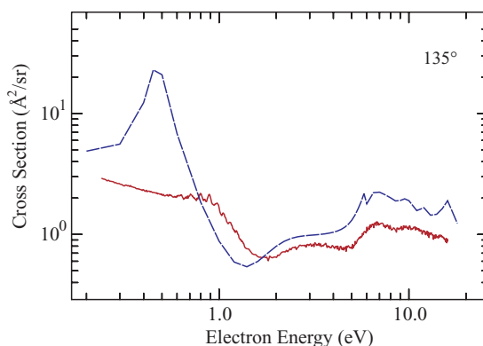
FIG. 4. (Color online) Elastic cross sections at 135^\circ .
