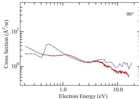
FIG. 3. (Color online) Elastic cross sections at 90^\circ .
