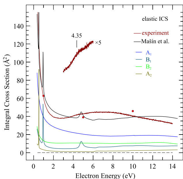
FIG. 8. Comparison of the experimental ICS with the calculated results (without Born correction) of Mašín et al. (Ref. 3 and this work). The contributions of all symmetries are indicated.
