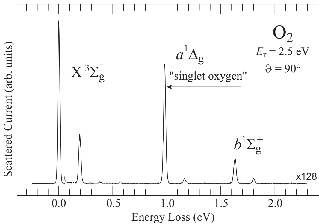
Fig. 1 A representative EEL-spectrum showing the “famous” singlet oxygen.
