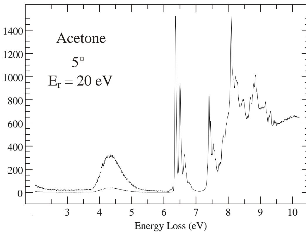
Fig. 1: Spectra emphasizing dipole-allowed transitions.
