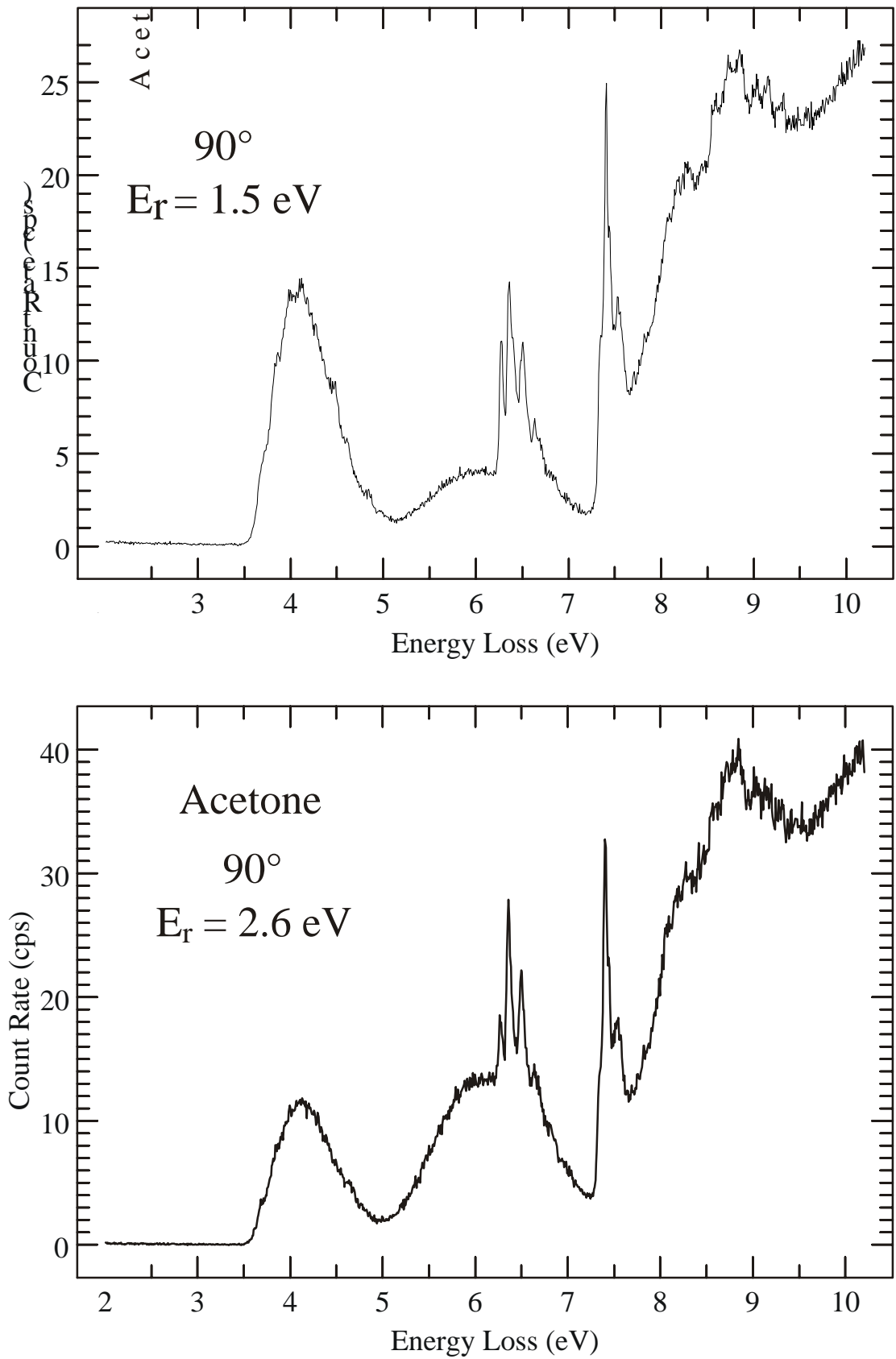
Fig. 2: Spectra emphasizing spin-forbidden transitions.
