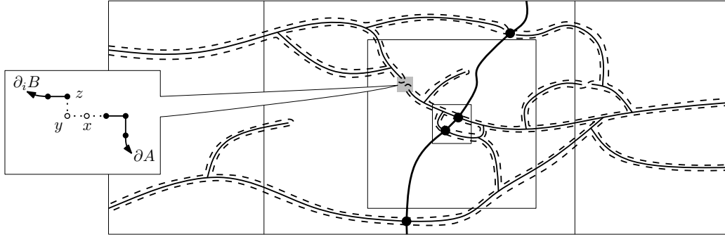
FIG 4. Two concentric balls A \subset B with two passage points in A but no passage points in B \setminus A . Note the three arms on either side of \gamma . The gray square marks the defect on one of the open arms.
