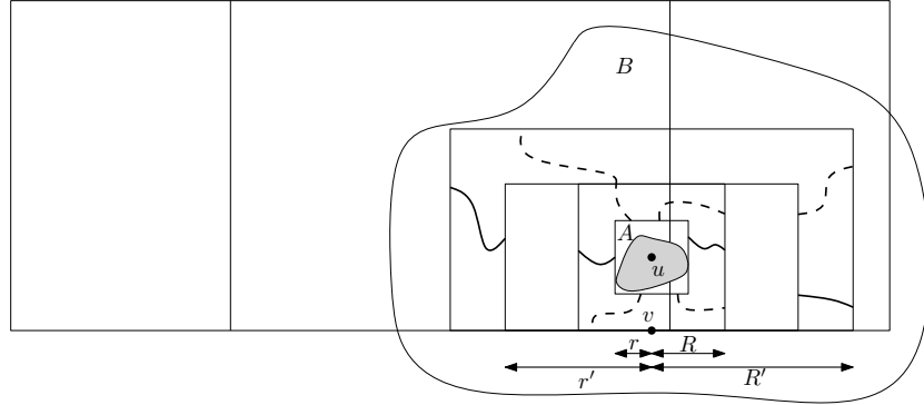
FIG 6. Two sets A \subset B intersecting R_n . The six arms between \partial\Lambda_r(u) and \partial_i\Lambda_R(u) and the four arms in \mathbb{H} between \partial\Lambda_{r'}(u) and \partial_i\Lambda_{R'}(u) ensure that \mathcal{E}(A, B) occurs.
