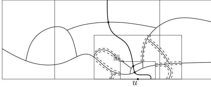
FIG 5. The intersection of \Lambda_r(u) with \mathbb{H} contains passage points, but \Lambda_R(u) \setminus \Lambda_r(u) does not. Then there are two open arms on either sides of \gamma between \partial\Lambda_r(u) and \partial_i\Lambda_R(u) . Above each open arm (but not necessarily also below) there is a closed arm.
