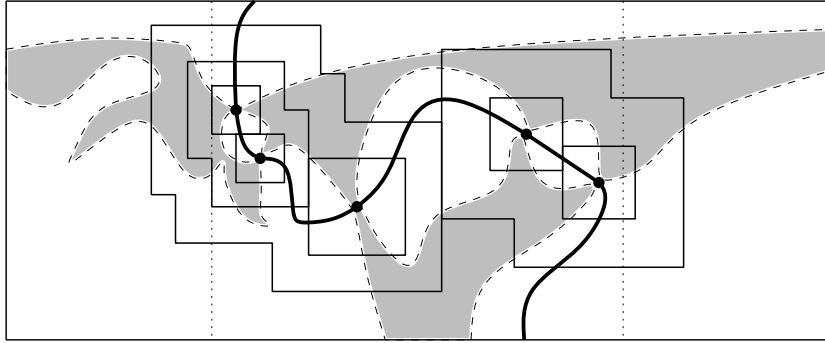
FIG 3. The crossing \gamma is drawn in bold and the passage points are marked. The set \chi of sites open in \omega but closed in \tilde{\omega} is drawn in gray. Its boundary is closed in \omega . The blobs at the times of merger are outlined. Observe the six arm structure between the boundaries of the blobs.
