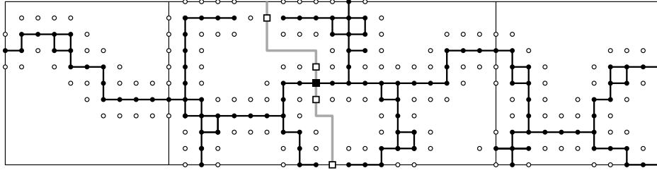
FIG 2. The set \chi in black, surrounded by \partial\chi . The gray path \gamma needs to use at least one passage point to cross \chi (black square). Even if a site which is pivotal for \{\omega \in \mathcal{C}_h(S_n)\} is enhanced, \gamma generally needs additional passage points to cross \partial\chi (see the empty squares).
