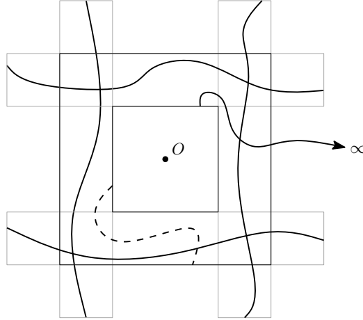
FIG 1. A situation with \omega \in C_n and \partial\Lambda_{n-1} \xleftrightarrow{\omega} \infty (the bold paths are open in \omega ) and such that there exists an \bar{\omega}^\sigma -open crossing of the annulus A(n, 2n) (dashed path). Then \bar{\omega}^\sigma \leq \tilde{\omega}^\sigma and there exists an \tilde{\omega}^\sigma -open crossing in the easy direction of one of the four rectangles forming A(n, 2n) . Note that any site of a \omega -open horizontal crossing of a gray rectangle is closed in \tilde{\omega} .
