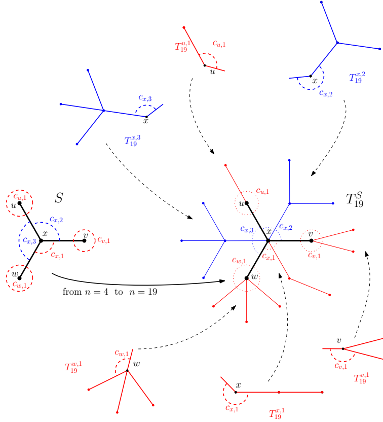
Figure 1: An example of decomposition into red and blue planted plane tree.
